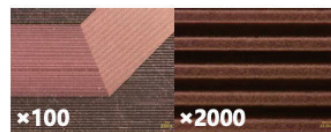
L/S = 15/15 μm
